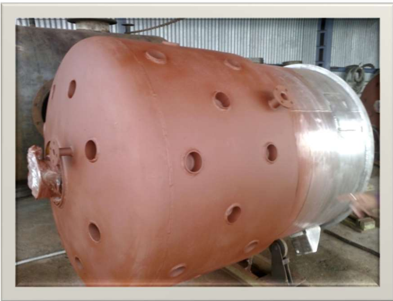
Jacketed Vessel
